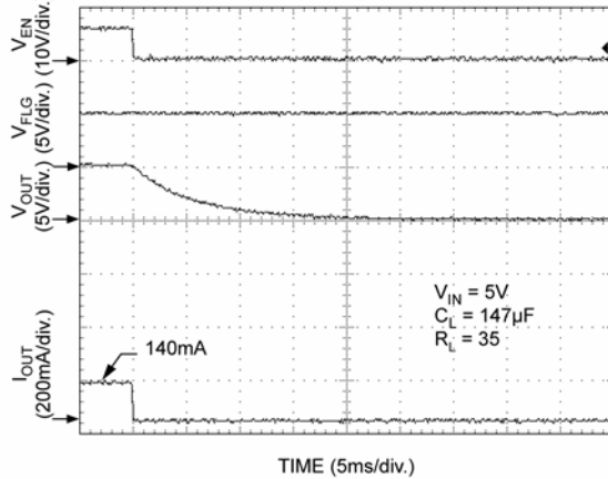
Turn-Off (MIC2026-1)
