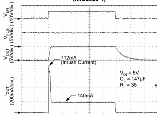
Turn-On/Turn-Off (MIC2026-1)
