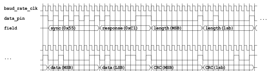
Figure 31-10. Example Response
