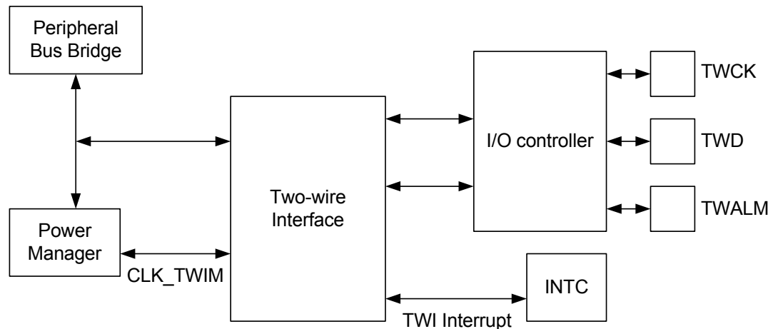
Figure 22-1. Block Diagram
