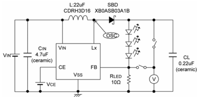
● Circuit ②
