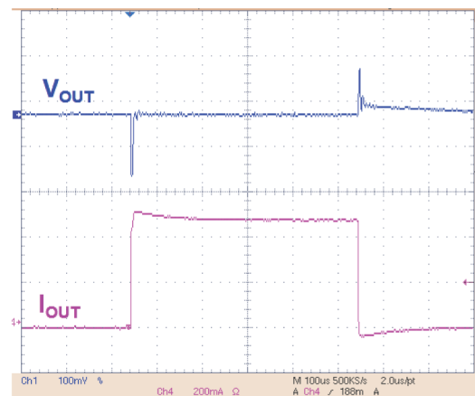
Figure 20. Load transient ( V_{BIAS} = 2.7\text{ V} , V_{IN} = 1.35\text{ V} ; I_{OUT} 1 to 500\text{ mA} )
