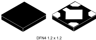
DFN4 1.2 x 1.2
