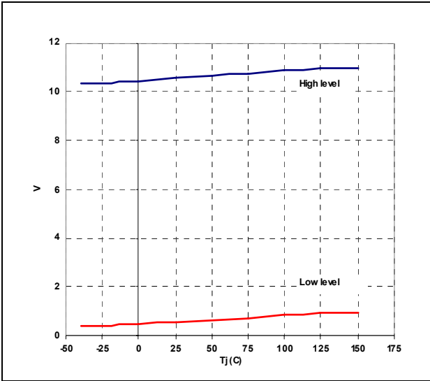
Figure 32. Gate drive output saturation vs T_J
