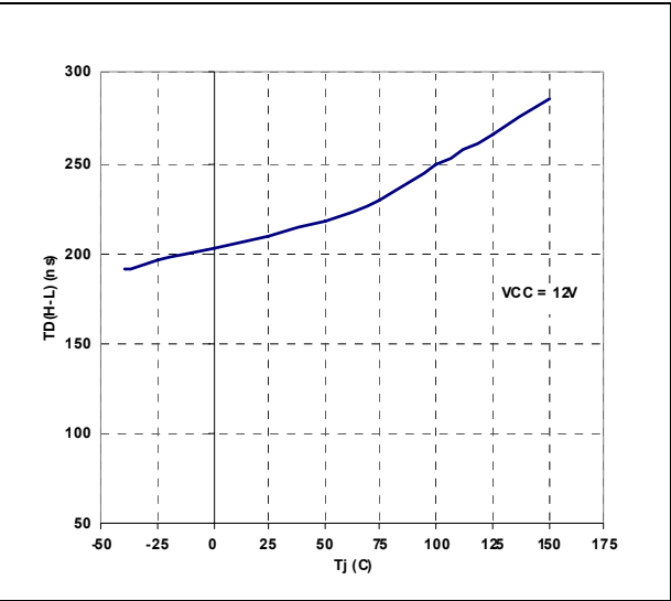
Figure 33. Delay to output vs T_J
