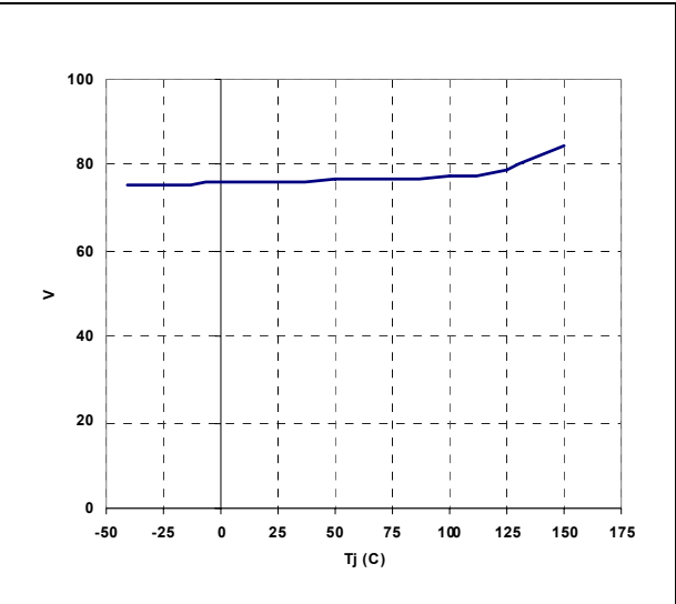
Figure 35. HV start voltage vs T_J
