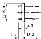
PCB Mounting Dimensions
