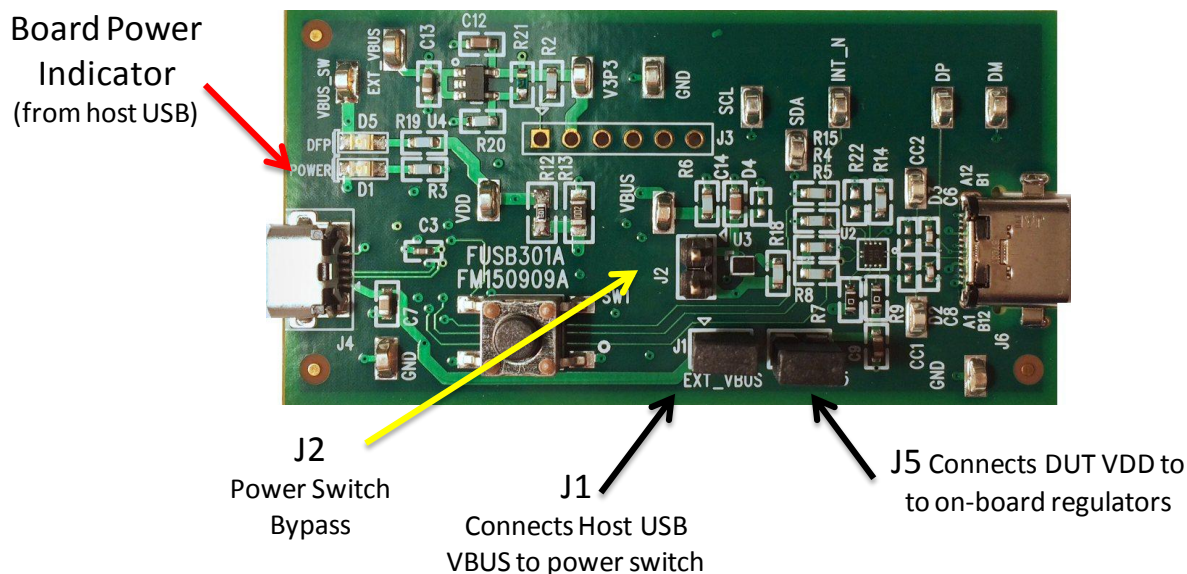
Figure 3 - FUSB301A Evaluation Board Power Configuration
