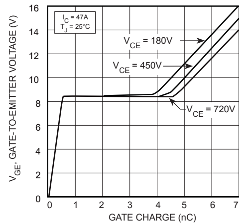
FIGURE 4, Gate charge
