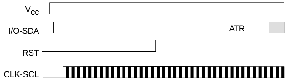
Figure 2. Asynchronous T = 0 Protocol
