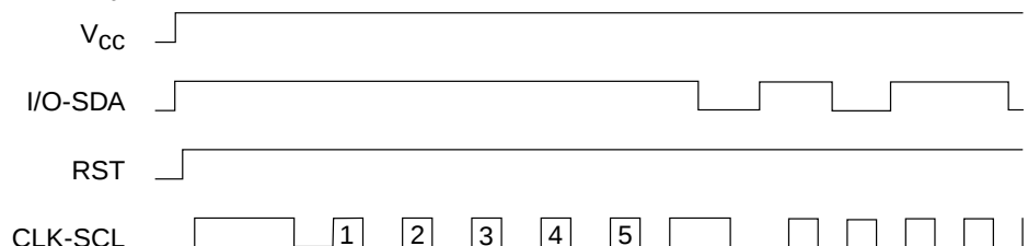
Figure 3. Synchronous 2-wire Protocol
