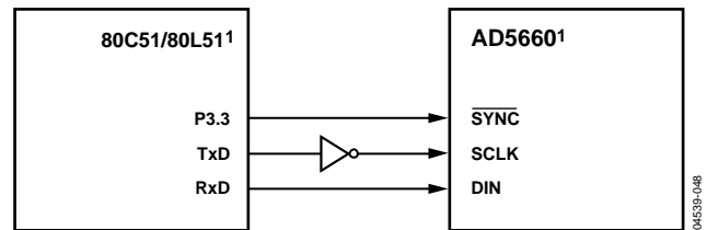
Figure 47. AD5660-to-80C51/80L51 Interface
