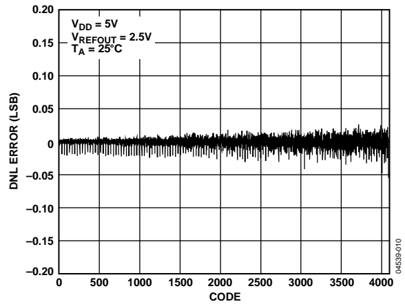
Figure 10. DNL—AD5620-2/AD6520-3
