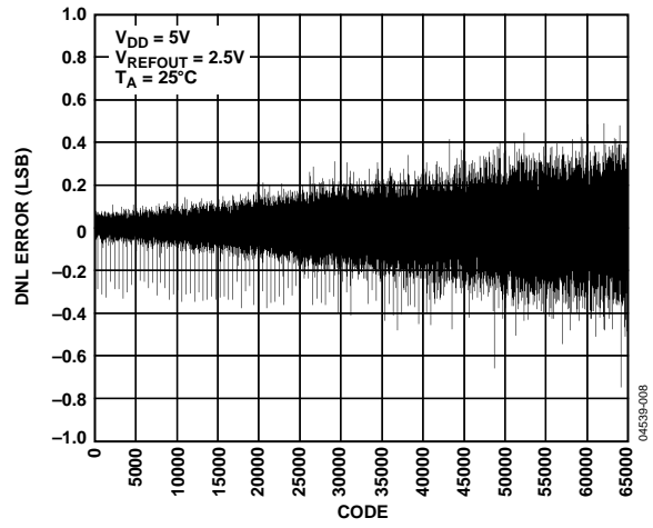
Figure 8. DNL—AD5660-2/AD5660-3
