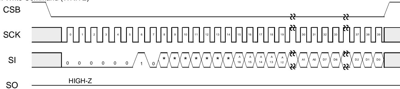
Figure 40. Write command
