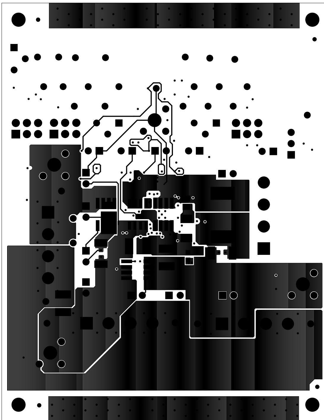
FIGURE 7. BOTTOM COPPER
