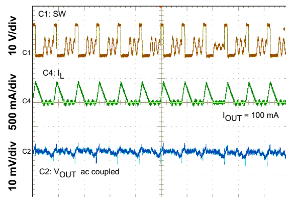
Figure 52. Output Ripple DCM
