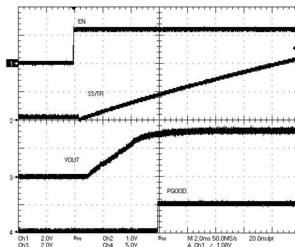
Figure 50. Startup With EN
