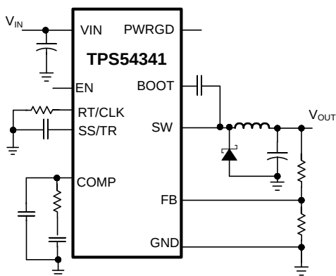
SIMPLIFIED SCHEMATIC
