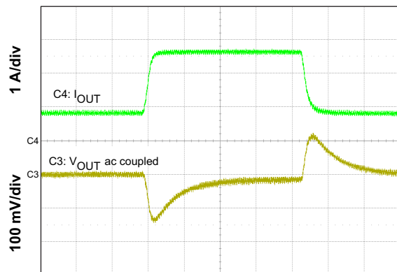
Figure 47. Load Transient
