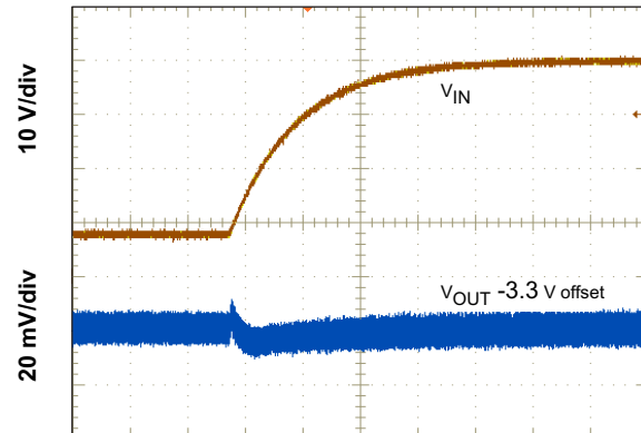
Figure 48. Line Transient (8 V to 40 V)
