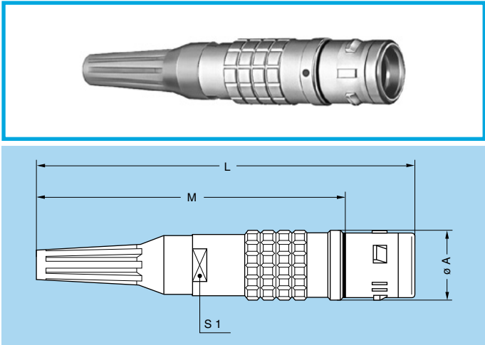
FGW.3K Straight plug, keys (W), cable adapter, with bend relief
