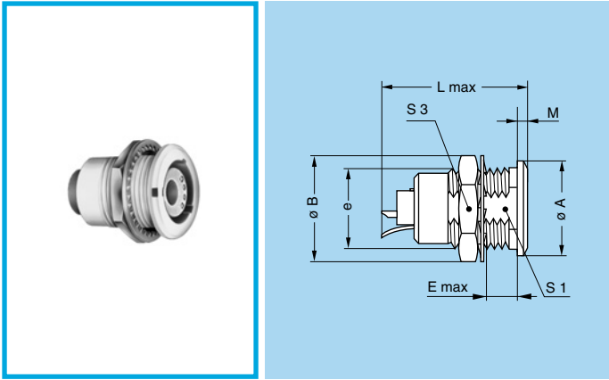
ENY Fixed socket with grounding tab, nut fixing, keys (Y), PSU or PPSU outer shell
