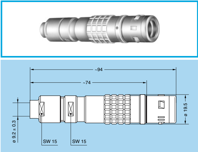
FUW.3K Straight plug, keys (W), cable collet adapter and long shell for fitting a bend relief with cap (with enhanced screen efficiency)
