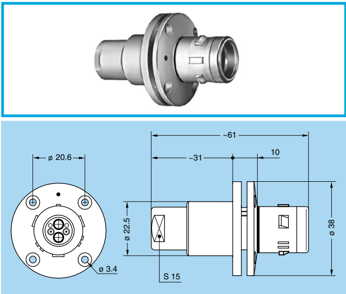
FXW.3K Fixed plug with round flange (4 holes fixing), keys (W)
