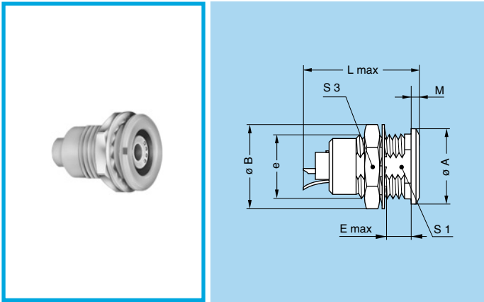
ENG Fixed socket with grounding tab, nut fixing, key (G or J), PEEK outer shell
