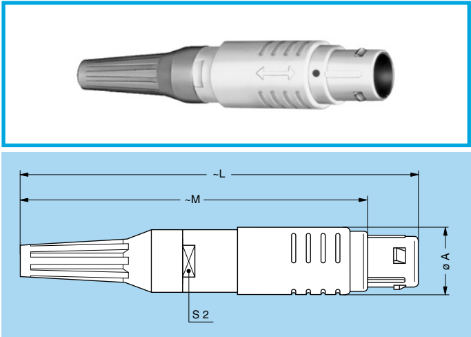
FGY Straight plug, keys (Y), cable collet and PSU or PPSU outer shell and nut for fitting a bend relief
