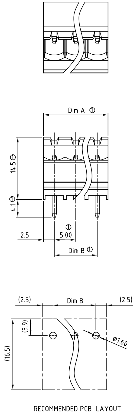
RECOMMENDED PCB LAYOUT
