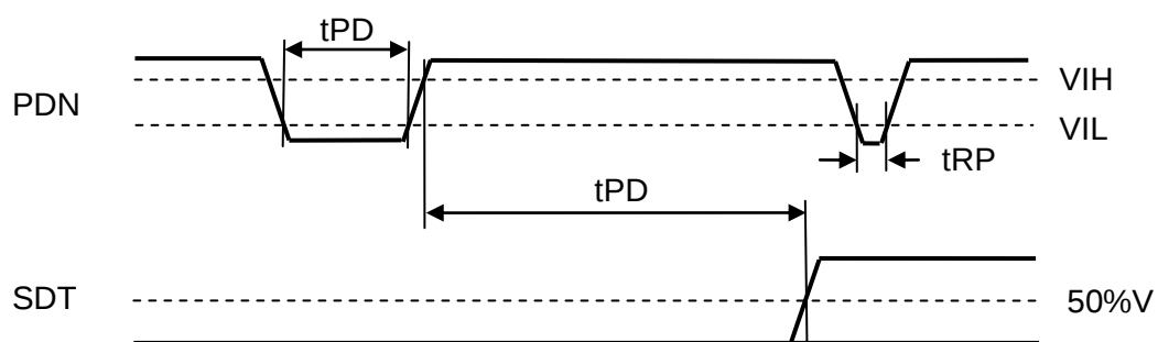
Figure 7. Power-down &amp; Reset Timing
