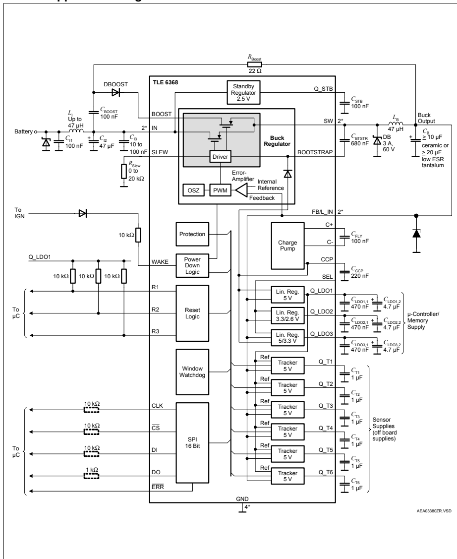
Figure 14 Application Diagram
