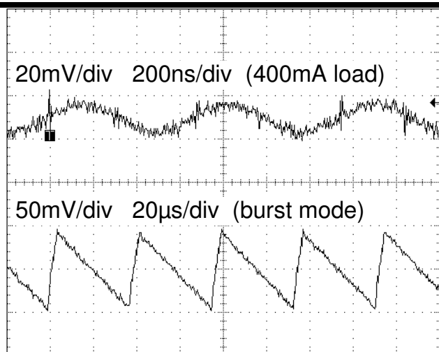
Figure 2. Output Ripple Voltage
