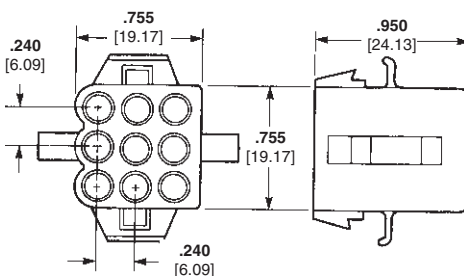
Socket Housing (Plug) Part No. 1-480672-0 Part No. 1586305-1 (Black Color High Temp.)
