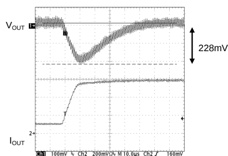
Conventional product (VOUT of which is 3.3 volts)
