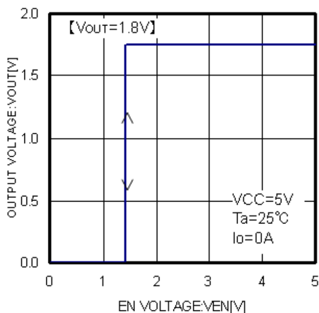
Figure 12. V_{OUT} VS V_{EN}
