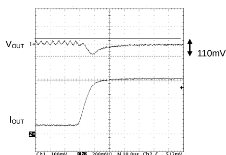
BD9106FVM-LB (Load response I_O=100mA \rightarrow 600mA )
