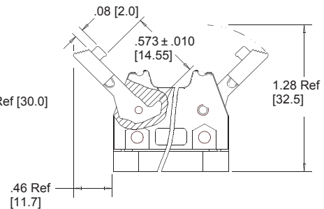
-D30X Header with Long Ejector/Latch for 3M Sockets with Strain Relief
