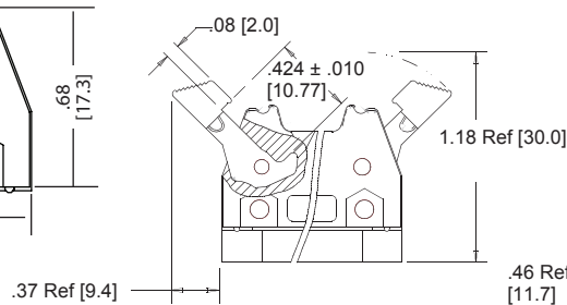
-D20X Header with Short Ejector/Latch for 3M Sockets without Strain Relief
