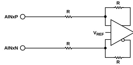
Figure 16. Analog Input Block
