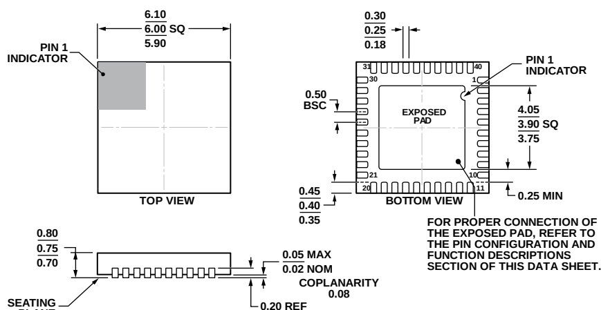
Figure 45. 40-Lead Lead Frame Chip Scale Package [LFCSP_WQ] 6 mm x 6 mm Body, Very Very Thin Quad (CP-40-14) Dimensions shown in millimeters
