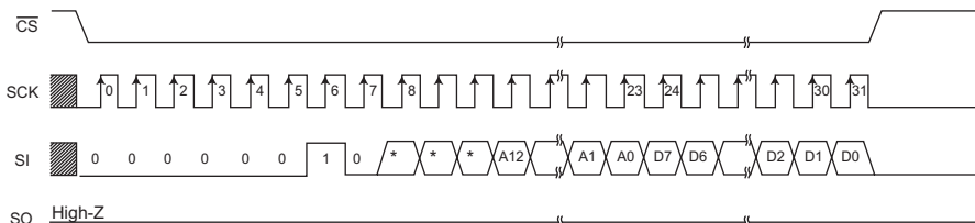
Fig.40 Write command (BR25L080/160/320/640-W) * =Don't care
