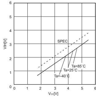
Fig.6 "H" input voltage V_{IH}(V_{CC}, SCK, SI, \overline{HOLD}, \overline{WP})
