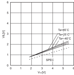
Fig.7 "L" input voltage V_{IL}(V_{CC}, SCK, SI, \overline{HOLD}, \overline{WP})
