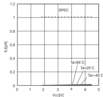
Fig.12 Input leak current I_{IL}(CS, SCK, SI, \overline{WP}, \overline{HOLD})
