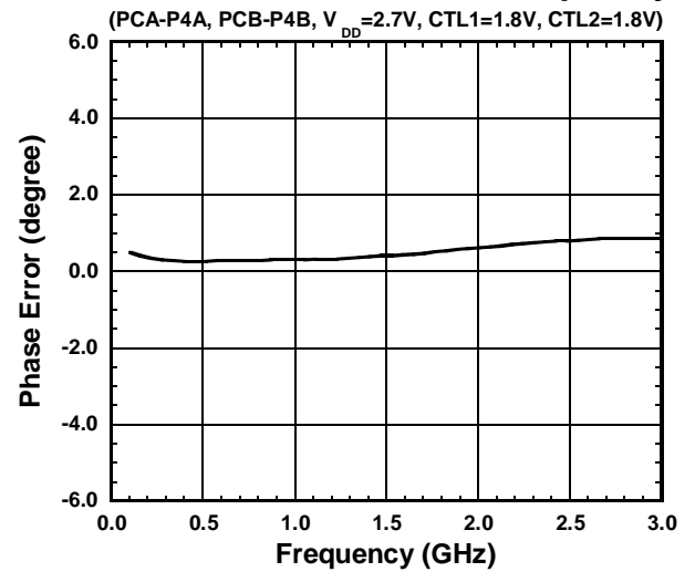
PC-P4 Phase Error vs. Frequency
