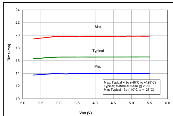
FIGURE 37-60: WDT Time-Out Period, PIC16F1773/6 Only.
