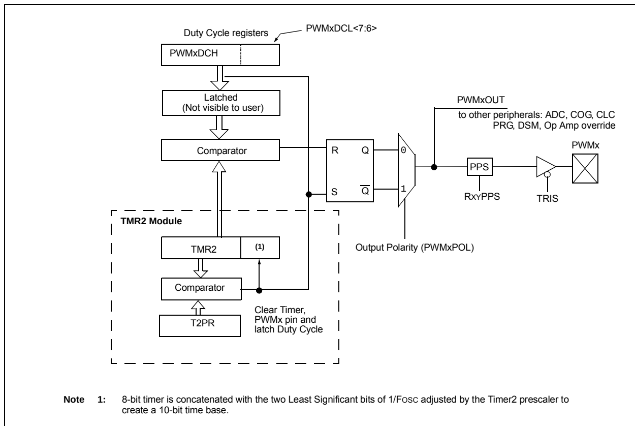
FIGURE 25-2: PWM OUTPUT
