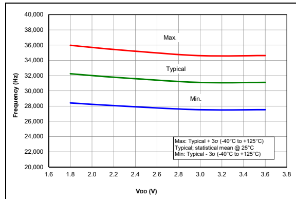
FIGURE 37-58: LFINTOSC Frequency, PIC16LF1773/6 Only.
