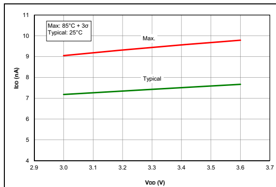
FIGURE 37-40: I_{DD} , Brown-Out Reset (BOR), BORV = 1, PIC16LF1773/6 Only.
