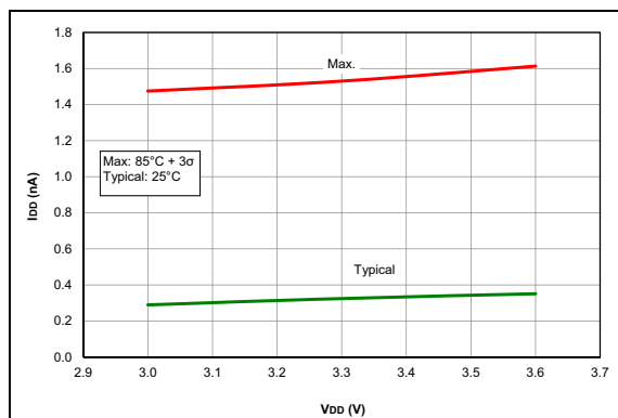
FIGURE 37-42: I_{DD} , LP Brown-Out Reset (LPBOR = 0), PIC16LF1773/6 Only.
