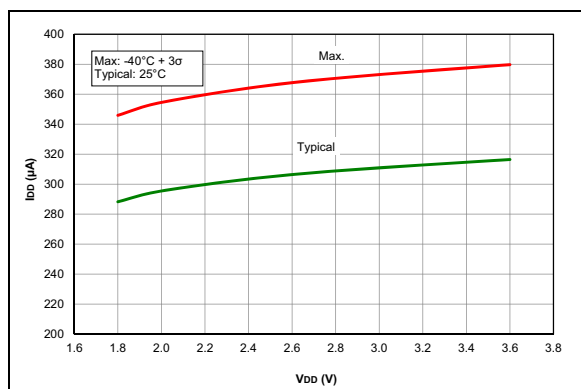
FIGURE 37-50: I_{PD} , Comparator, NP Mode ( V_{REGPM} = 0 ), PIC16LF1773/6 Only.
