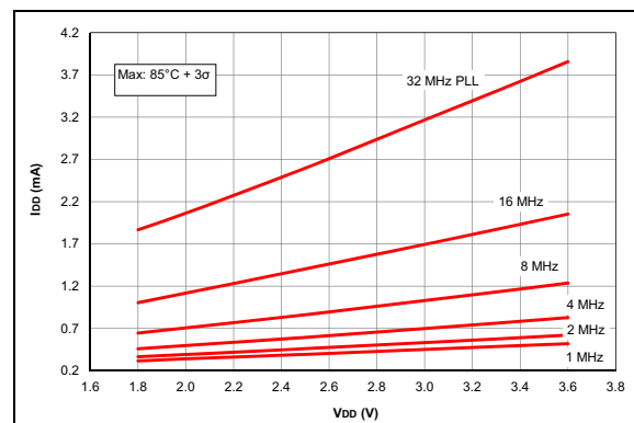
FIGURE 37-24: I_{DD} Maximum, HFINTOSC Mode, PIC16LF1773/6 Only.
