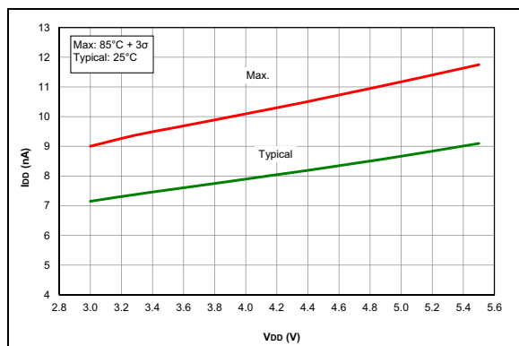
FIGURE 37-41: I_{PD} , Brown-Out Reset (BOR), BORV = 1, PIC16F1773/6 Only.
