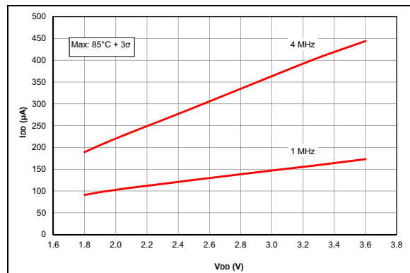
FIGURE 37-12: I_{DD} Maximum, EC Oscillator MP Mode, PIC16F1773/6 Only.
