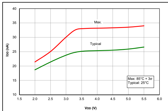
FIGURE 37-39: I_{PD} , Fixed Voltage Reference (FVR), DAC/Comparator, PIC16F1773/6 Only.
