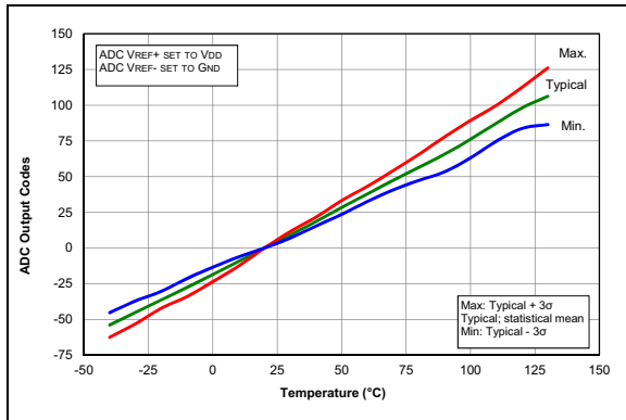
FIGURE 37-91: Temperature Indicator Slope Normalized to 20°C, Low Range, V_{DD} = 3.0V , PIC16F1773/6 only.
