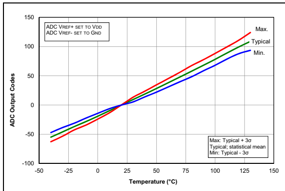
FIGURE 37-93: Temp. Indicator Slope Normalized to 20°C, Low Range, V_{DD} = 3.0V , PIC16LF1773/6 Only.
