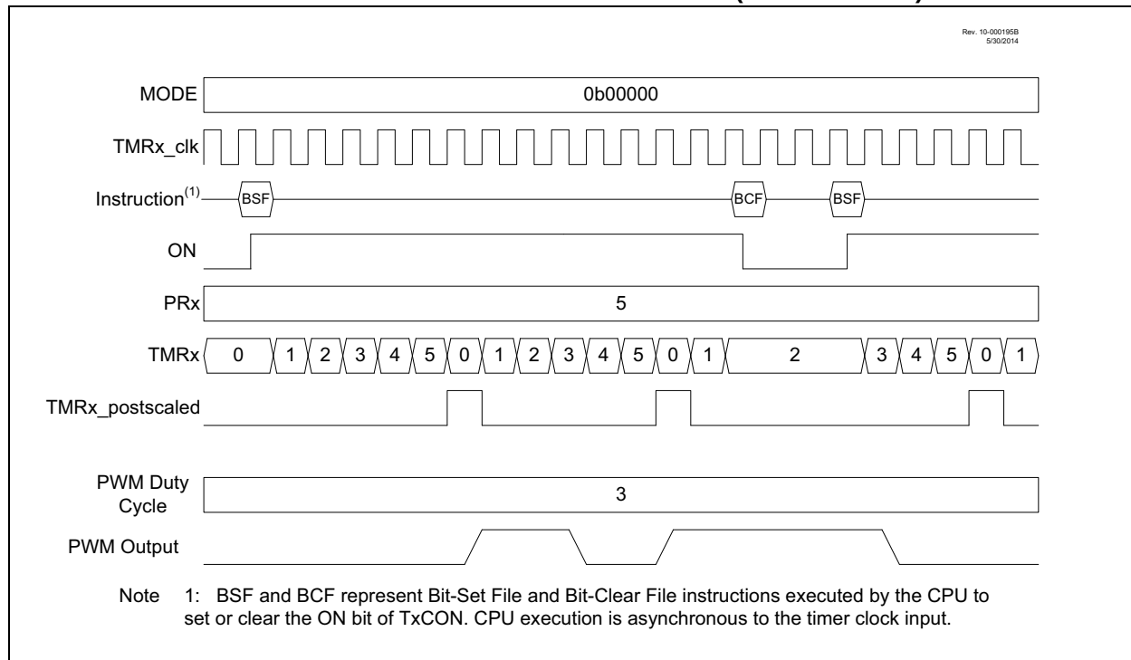
FIGURE 23-4: SOFTWARE GATE MODE TIMING DIAGRAM (MODE = 000000)
