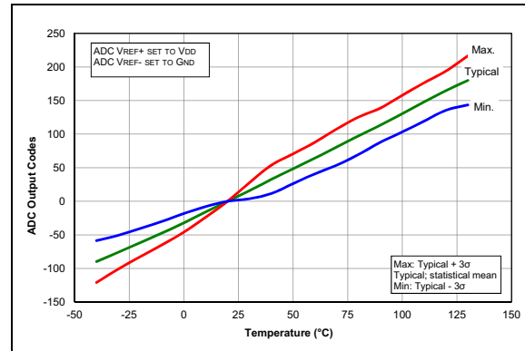
FIGURE 37-92: Temp. Indicator Slope Normalized to 20°C, Low Range, V_{DD} = 1.8V , PIC16LF1773/6 Only.
