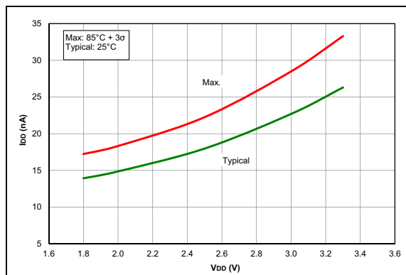
FIGURE 37-38: I_{PD} , Fixed Voltage Reference (FVR), DAC/Comparator, PIC16LF1773/6 Only.
