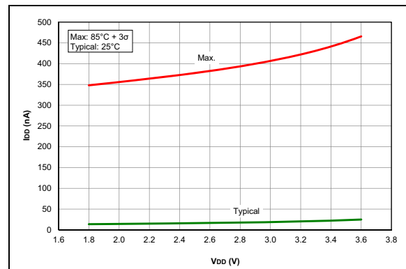
FIGURE 37-48: I_D , ADC Non-Converting, PIC16LF1773/6 Only.
