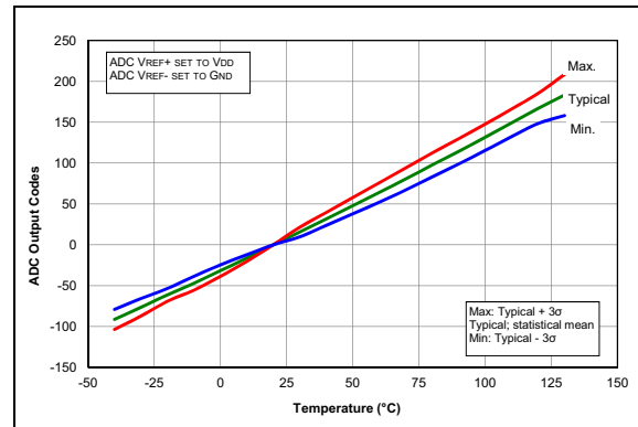
FIGURE 37-94: Temp. Indicator Slope Normalized to 20°C, High Range, V_{DD} = 3.6V , PIC16LF1773/6 Only.
