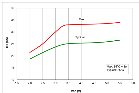
FIGURE 37-37: I_{PD} , Fixed Voltage Reference (FVR), ADC, PIC16F1773/6 Only.
