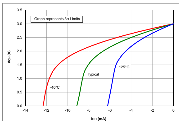
FIGURE 37-54: V_{OL} vs. I_{OH} Over Temperature, V_{DD} = 3.0V .
