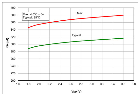
FIGURE 37-50: I_{D} , Comparator, NP Mode ( V_{REGPM} = 0 ), PIC16LF1773/6 Only.
