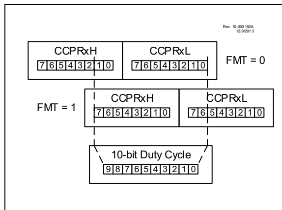
FIGURE 24-4: CCPx DUTY CYCLE ALIGNMENT
