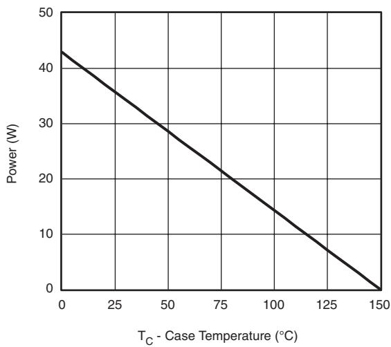
Power, Junction-to-Case
