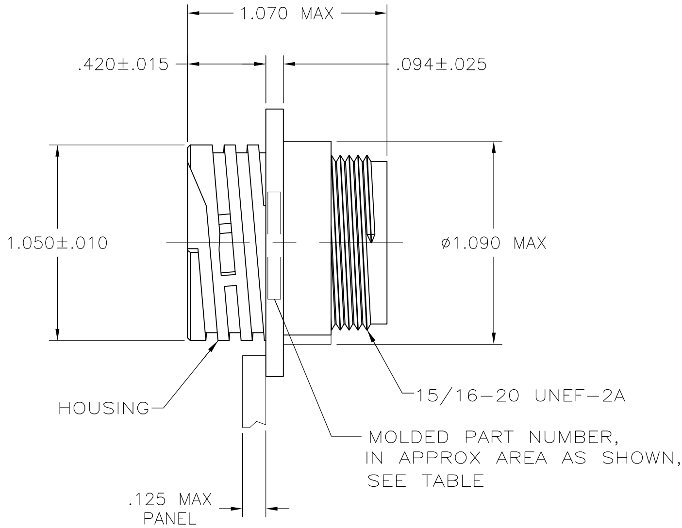
DETAIL A
