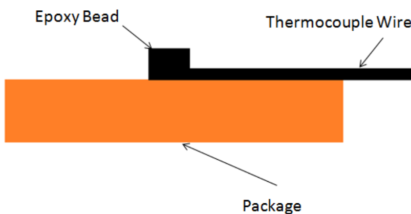
Figure 12-16. Technique for Measuring T_{case} with 0° Angle Attachment, No Heat Sink
