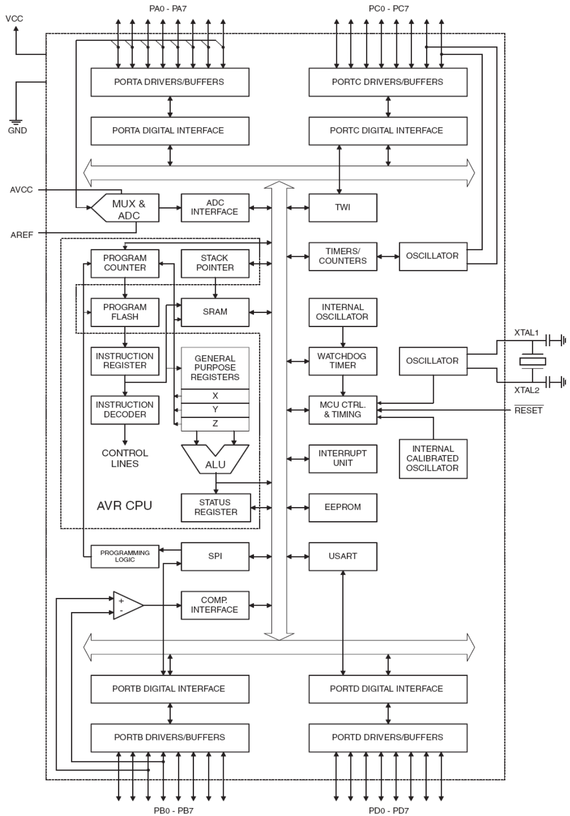
Figure 2. Block Diagram
