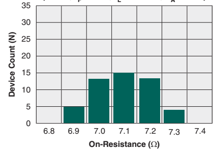
Typical On-Resistance Distribution (N=50, I_F=1\text{mA} , I_L=120\text{mA} , T_A=25^\circ\text{C} )
