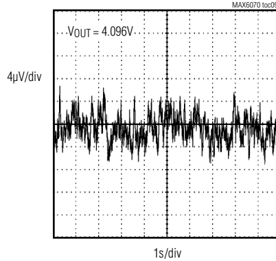
MAX6070_41 OUTPUT NOISE (0.1Hz TO 10Hz)
