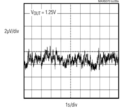
MAX6070_12 OUTPUT NOISE (0.1Hz TO 10Hz)
