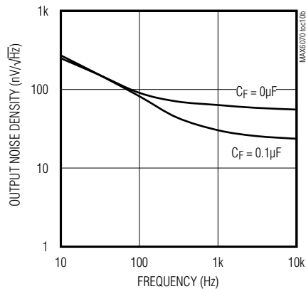
MAX6070_25 OUTPUT NOISE DENSITY vs. FREQUENCY
