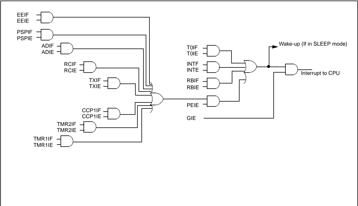
FIGURE 11-9: INTERRUPT LOGIC
