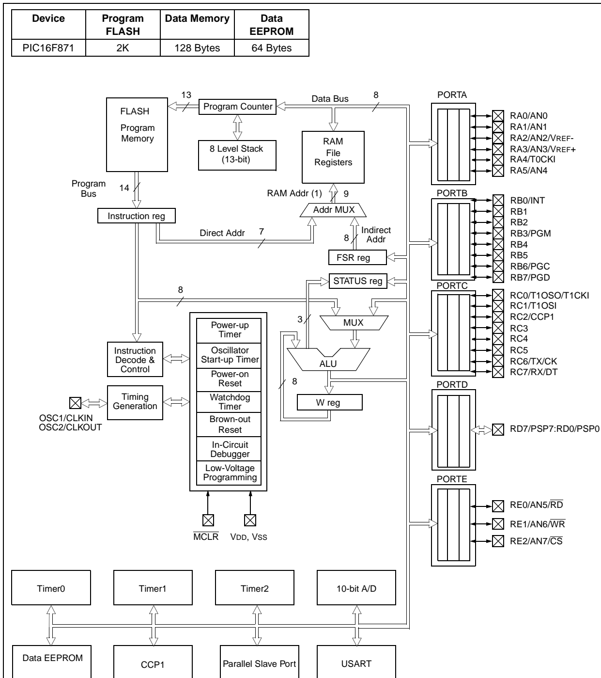
FIGURE 1-2: PIC16F871 BLOCK DIAGRAM
