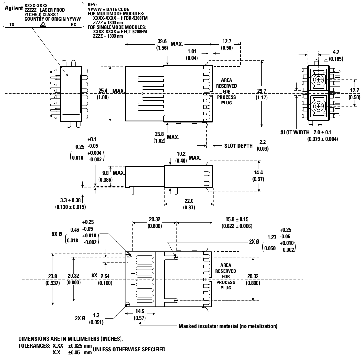
Figure 10. Package Outline for HFBR/HFCT-5208FM
