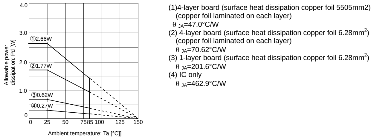
Figure 55. Thermal Derating Characteristics (VQFN016V3030)
