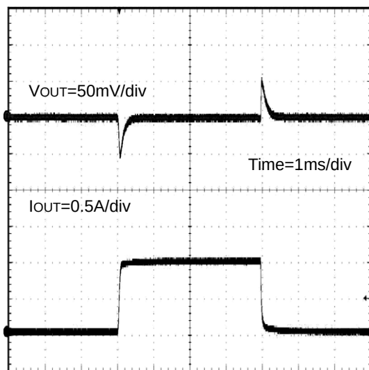
Figure 39. Load Transient Response I_{OUT}=0A to 1A load step ( V_{IN}=5V , V_{OUT}=1.8V , C_{OUT} =Ceramic 44\mu F )
