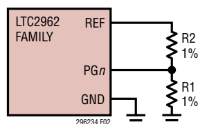
Figure 2. Monitor Configuration
