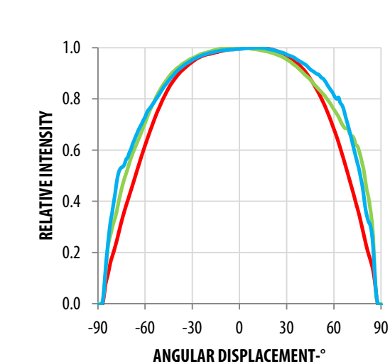
Figure 5: Radiation Pattern
