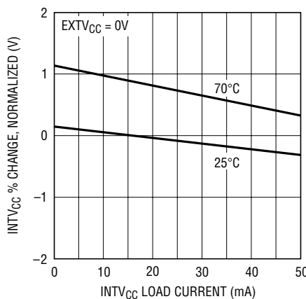
INTV CC Regulation vs INTV CC Load Current
