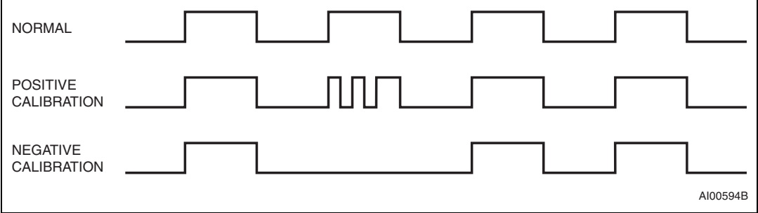
Figure 11. Clock calibration
