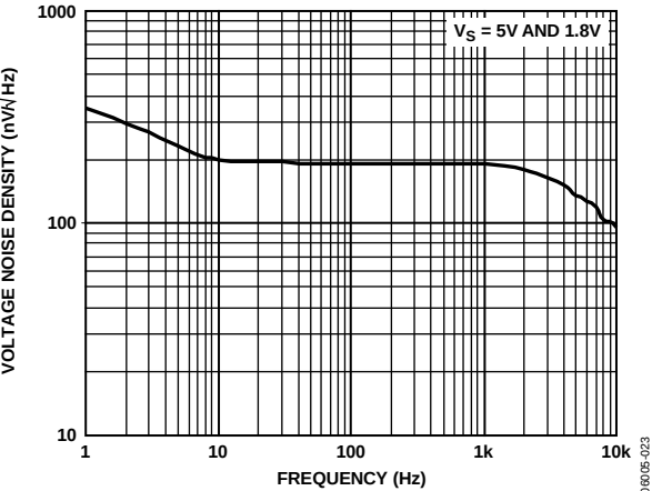
Figure 23. Voltage Noise Density
