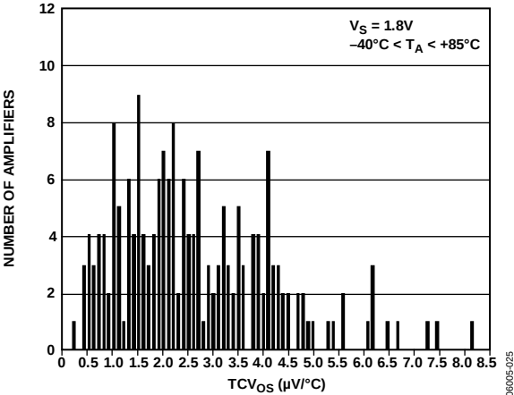
Figure 25. Input Offset Voltage Drift Distribution
